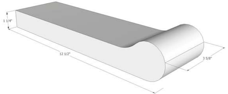
ISOMETRIC VIEW
