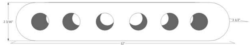
ELEVATION VIEW
