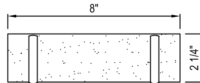
ELEVATION VIEW
